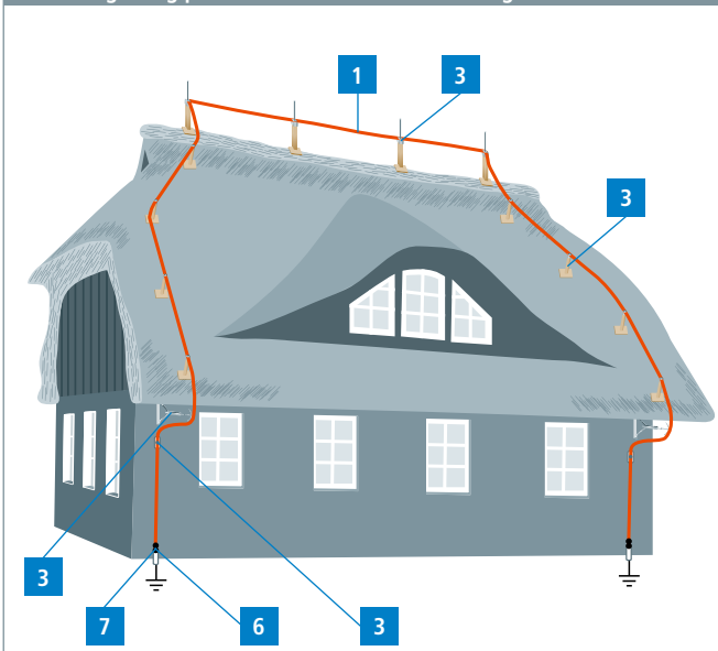
External lightning protection of a residential building with a thatched roof
