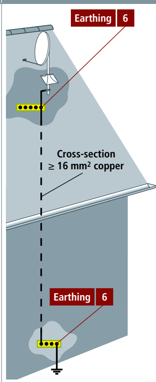
Equipotential bonding inside a building without a lightning protection system
